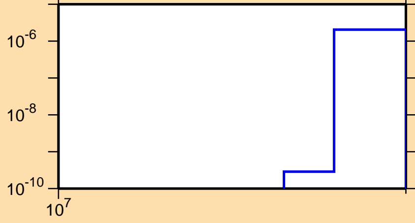
\sigma vs. E for ^{170}\text{Yb}(n,2np)
