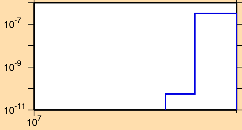
\sigma vs. E for ^{170}\text{Yb}(n,nt)
