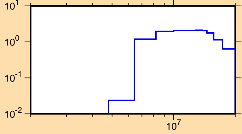
\sigma vs. E for ^{169}\text{Er}(n,2n)
