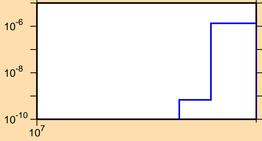
\sigma vs. E for ^{171}\text{Er}(n,nt)
