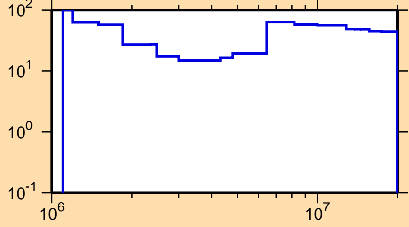
\Delta\sigma/\sigma vs. E for ^{171}\text{Er}(n,n\text{cont.})
