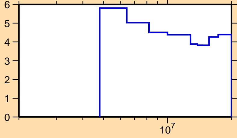
\Delta\sigma/\sigma vs. E for ^{160}\text{Tb}(n,\text{nonel.})
