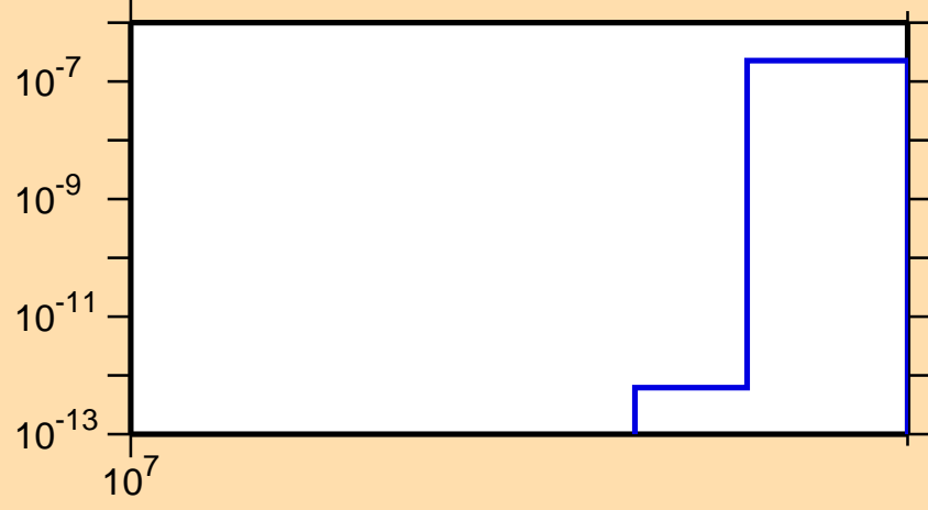
\sigma vs. E for ^{158}\text{Dy}(n,2np)
