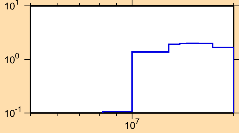
\sigma vs. E for ^{158}\text{Dy}(n,2n)
