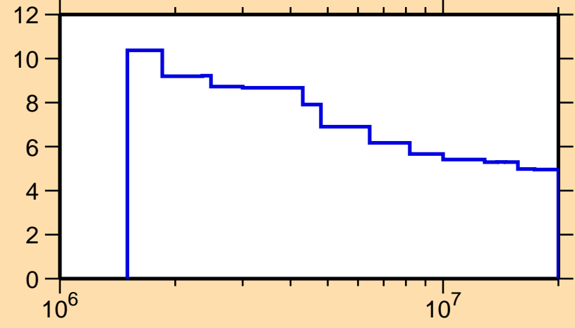
\Delta\sigma/\sigma vs. E for ^{158}\text{Dy}(n,nonel.)
