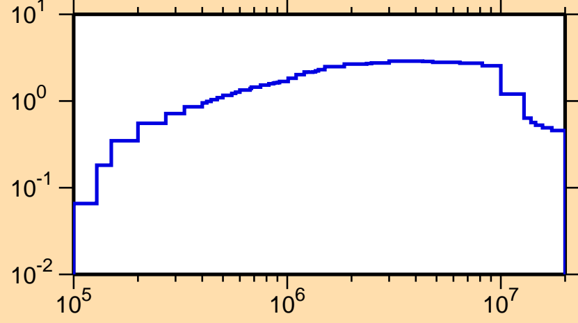
\sigma vs. E for ^{158}\text{Dy}(n,\text{inel.})
