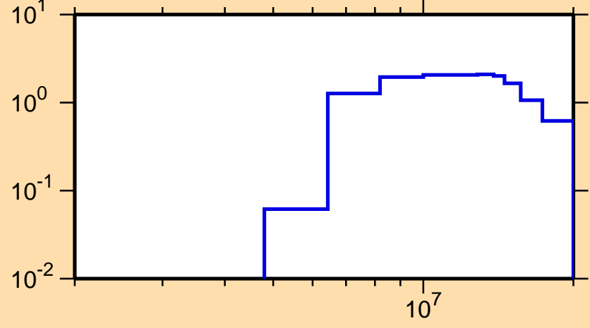
\sigma vs. E for ^{165}\text{Dy}(n,2n)
