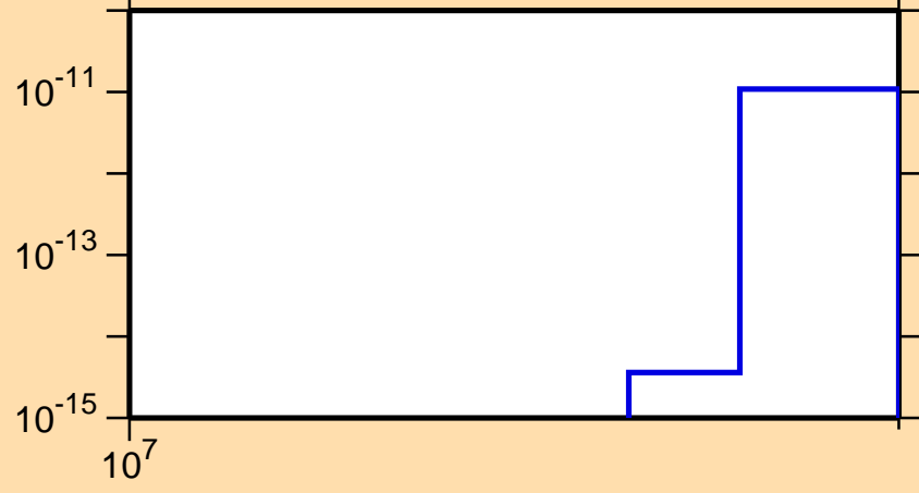
\sigma vs. E for ^{165}\text{Dy}(n,\text{He3})
