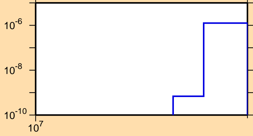
\sigma vs. E for ^{165}\text{Dy}(n,2np)
