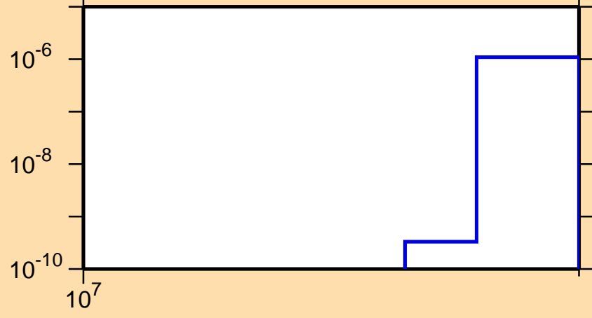
\sigma vs. E for ^{165}\text{Dy}(n,nt)
