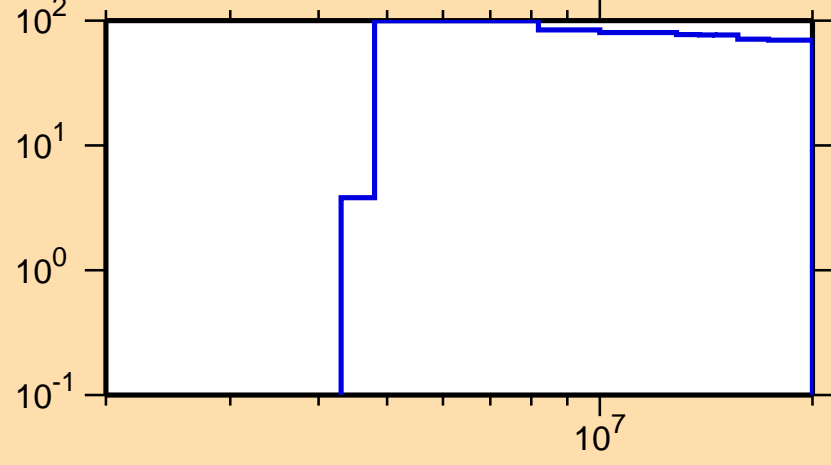
\Delta\sigma/\sigma vs. E for ^{165}\text{Dy}(n,p)
