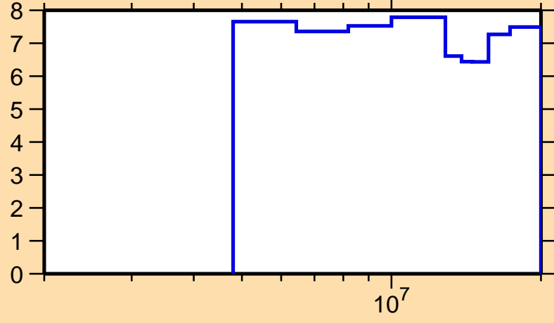
\Delta\sigma/\sigma vs. E for ^{165}\text{Dy}(n,\text{nonel.})
