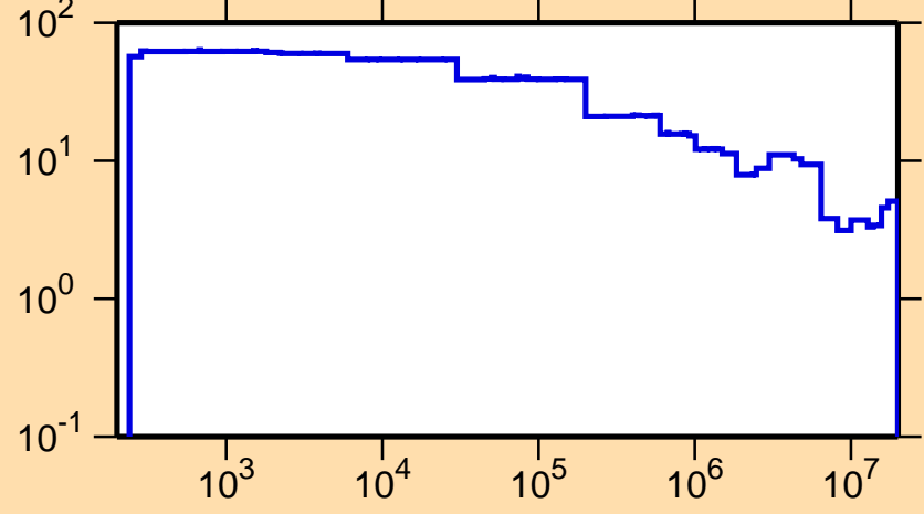
\Delta\sigma/\sigma vs. E for ^{166}\text{Ho}(n,\text{tot.})
