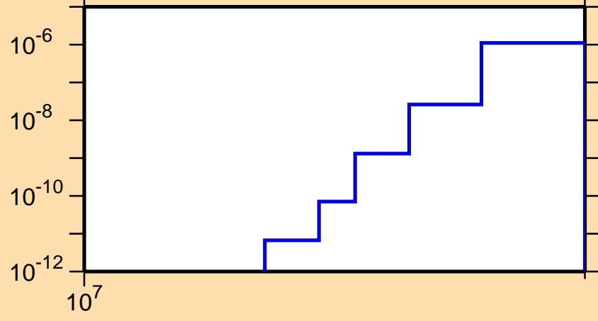
\sigma vs. E for ^{151}\text{Gd}(n,\text{He3})
