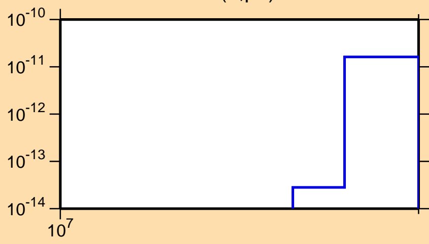
\sigma vs. E for ^{151}\text{Gd}(n,pd)
