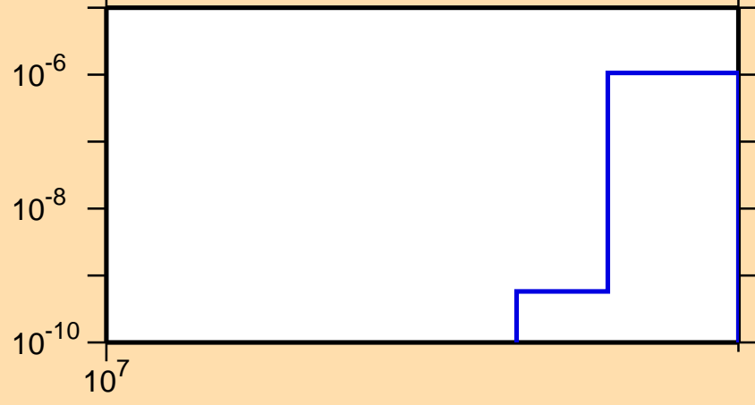
\sigma vs. E for ^{151}\text{Gd}(n,nt)
