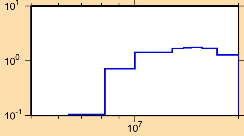
\sigma vs. E for ^{151}\text{Gd}(n,2n)
