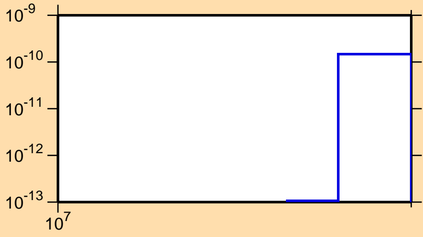
\sigma vs. E for ^{151}\text{Gd} (mt 34)
