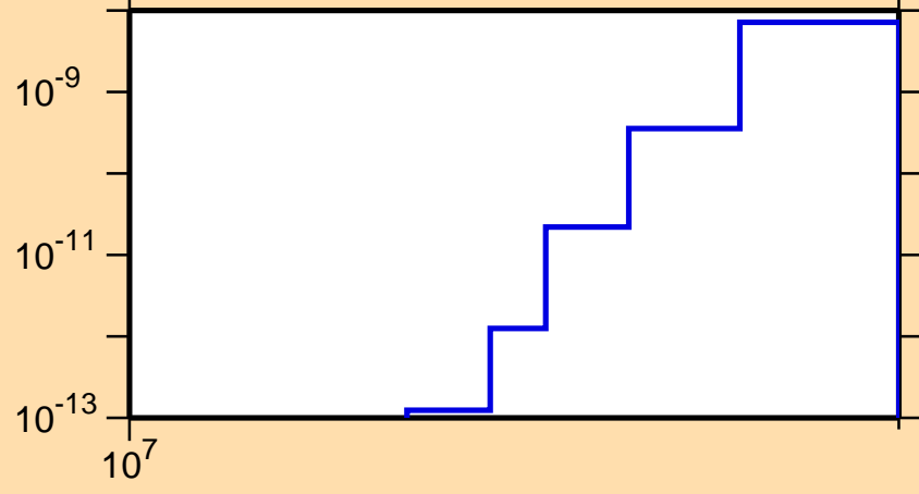
\sigma vs. E for ^{151}\text{Gd}(\text{mt117})
