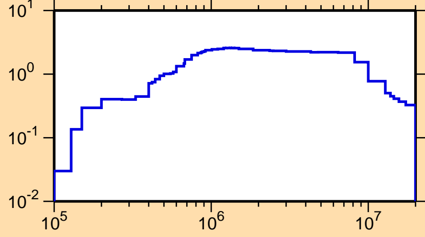
\sigma vs. E for ^{151}\text{Gd}(n,\text{inel.})
