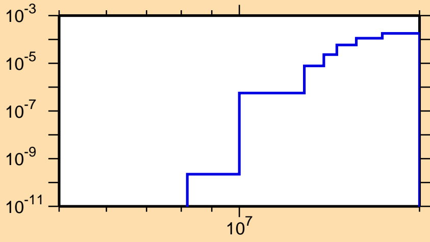
\sigma vs. E for ^{153}\text{Gd}(n,2n\alpha)
