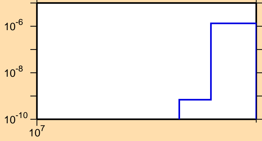
\sigma vs. E for ^{153}\text{Gd}(n,nt)
