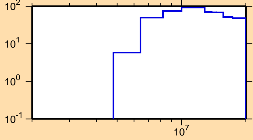
\Delta\sigma/\sigma vs. E for ^{153}\text{Gd}(n,\text{inel.})
