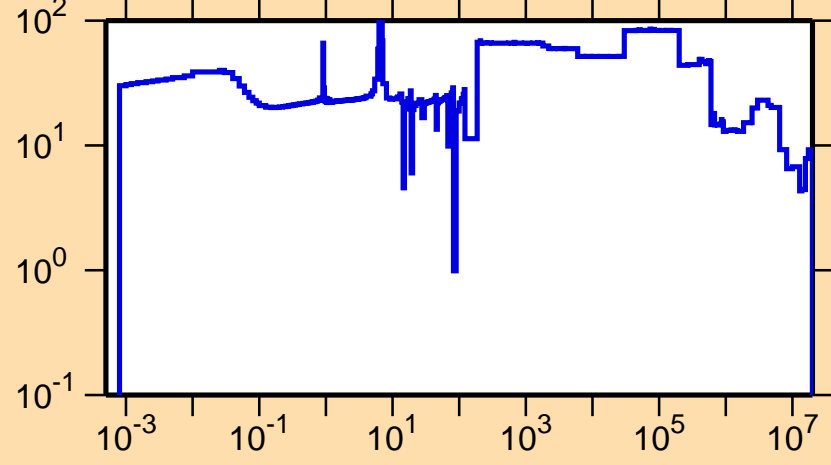
\Delta\sigma/\sigma vs. E for ^{153}\text{Gd}(n,\text{el.})
