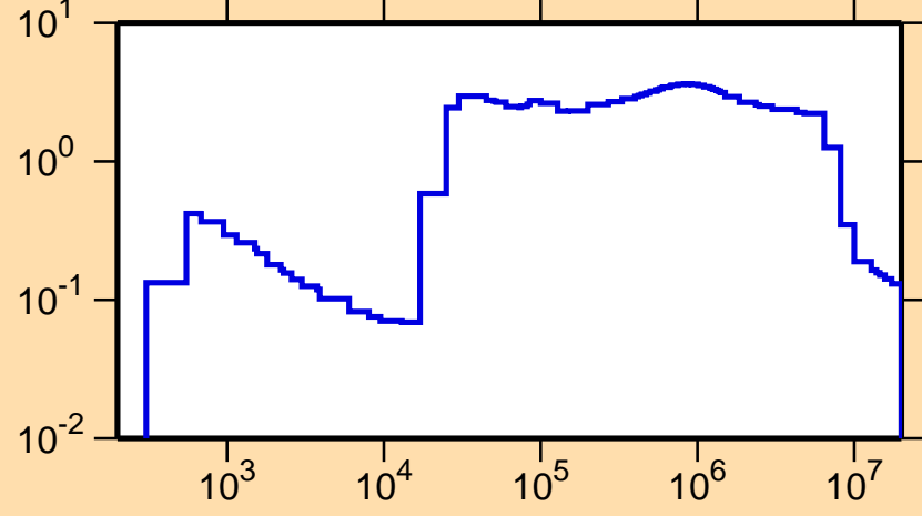
\sigma vs. E for ^{152}\text{Eu}(n,\text{inel.})
