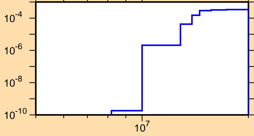
\sigma vs. E for ^{152}\text{Eu}(n,2n\alpha)
