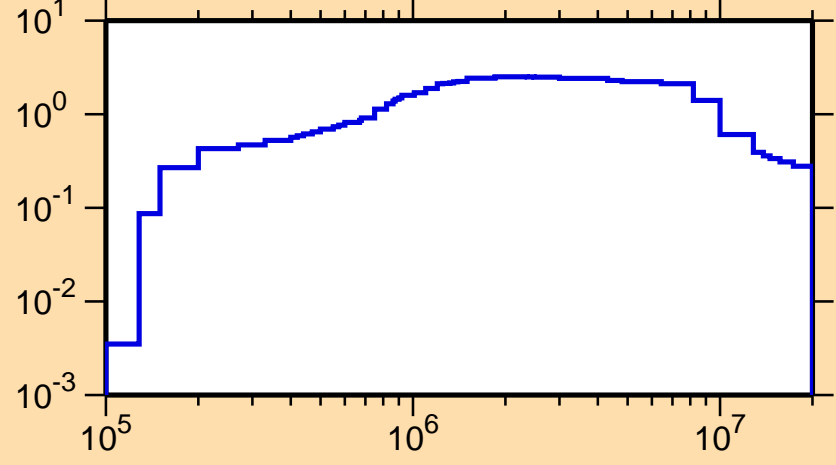
\sigma vs. E for ^{147}\text{Sm}(n,\text{inel.})
