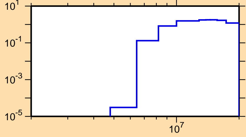
\sigma vs. E for ^{147}\text{Sm}(n,2n)
