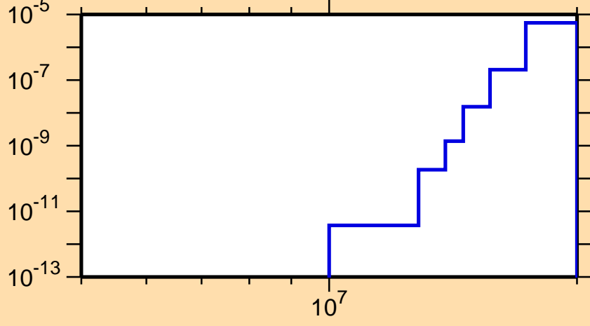
\sigma vs. E for ^{149}\text{Gd}(n,\text{He}3)
