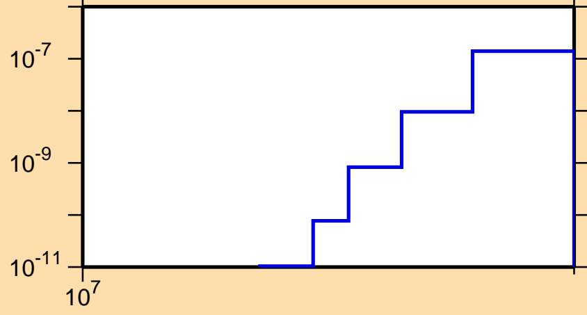
\sigma vs. E for ^{149}\text{Gd}(\text{mt117})
