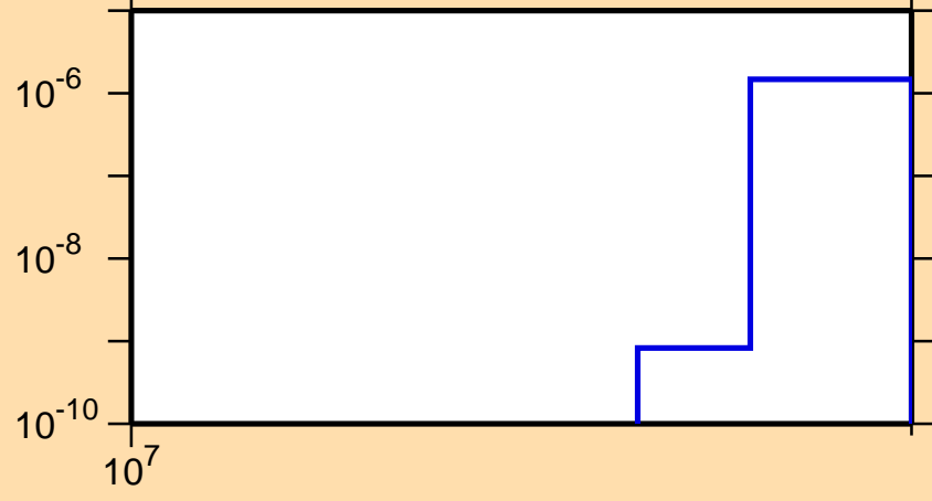
\sigma vs. E for ^{149}\text{Gd}(n,nt)
