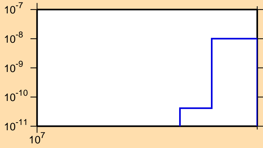
\sigma vs. E for ^{149}\text{Gd}(n,\text{pt})
