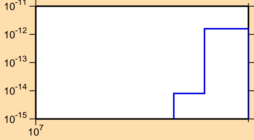
\sigma vs. E for ^{149}\text{Gd}(n,3n\alpha)
