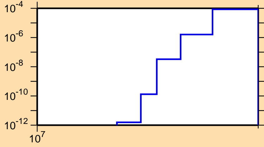
\sigma vs. E for ^{149}\text{Gd}(n,\text{nd})
