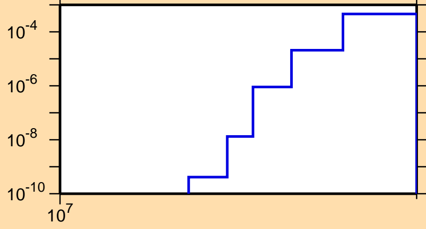
\sigma vs. E for ^{148}\text{Pm}(n,2np)
