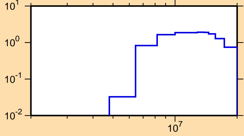
\sigma vs. E for ^{148}\text{Pm}(n,2n)
