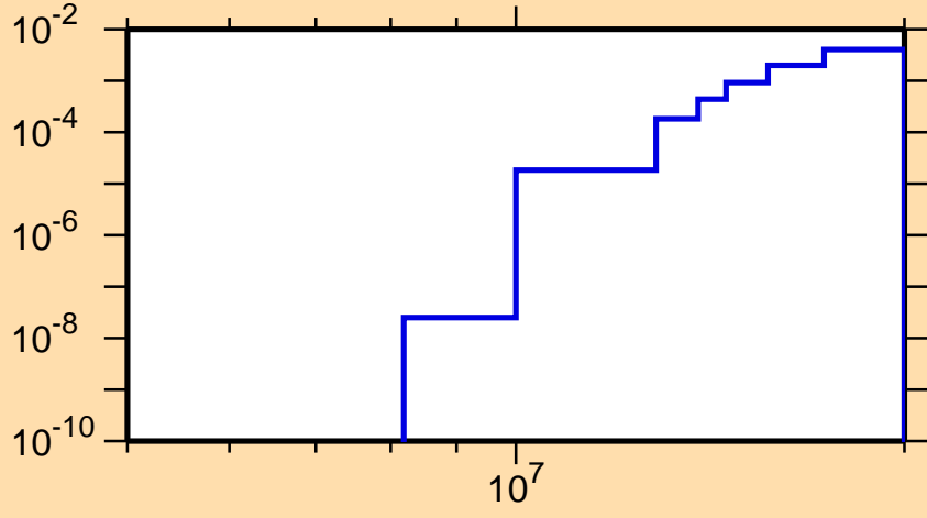
\sigma vs. E for ^{148}\text{Pm}(n,t)
