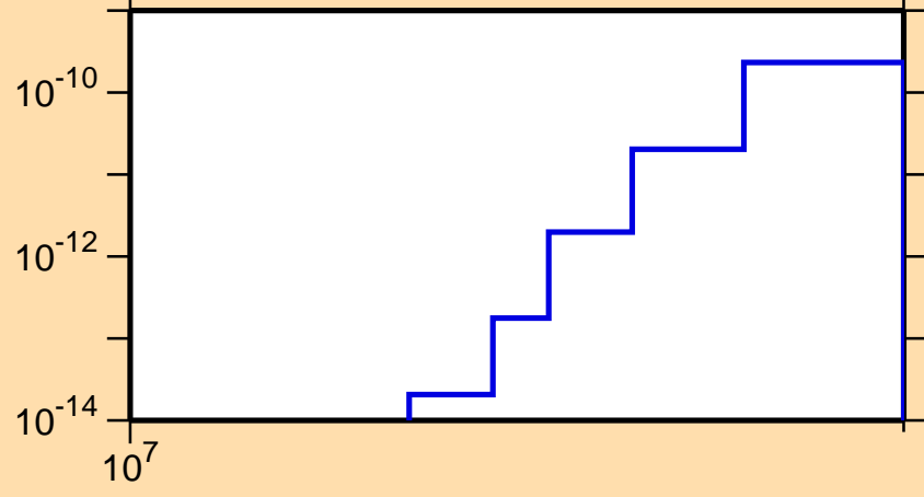
\sigma vs. E for ^{148}\text{Pm}(\text{mt117})
