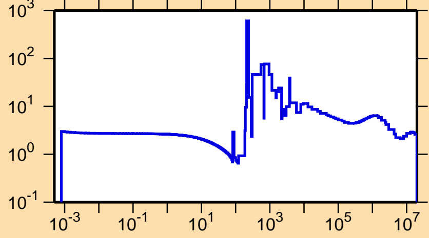
\sigma vs. E for ^{141}\text{Pr}(n,\text{el.})
