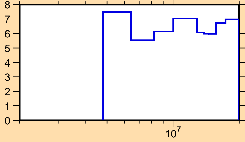
\Delta\sigma/\sigma vs. E for ^{143}\text{Ce}(n,\text{nonel.})
