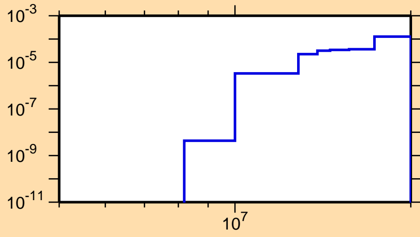
\sigma vs. E for ^{143}\text{Ce}(n,2n\alpha)
