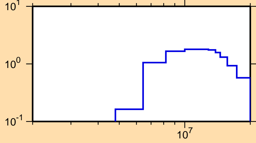
\sigma vs. E for ^{143}\text{Ce}(n,2n)
