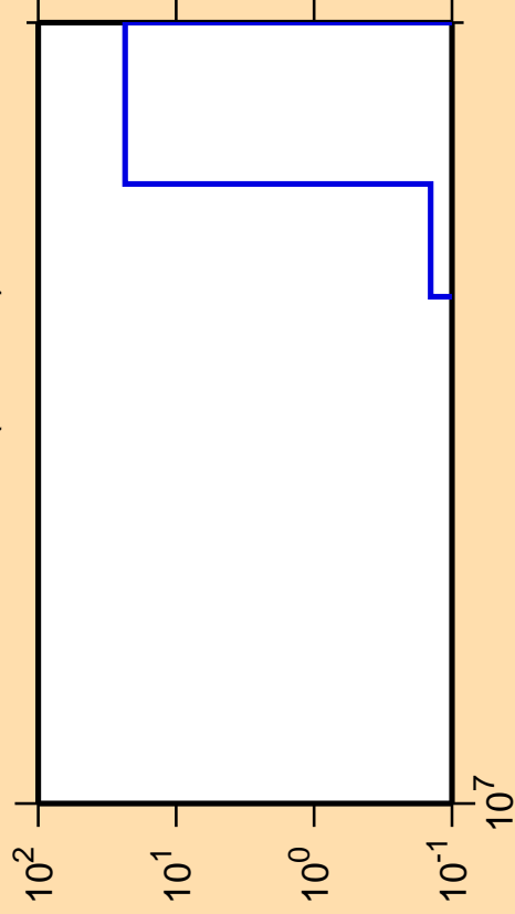
\Delta\sigma/\sigma vs. E for ^{143}\text{Ce}(\text{mt117})
