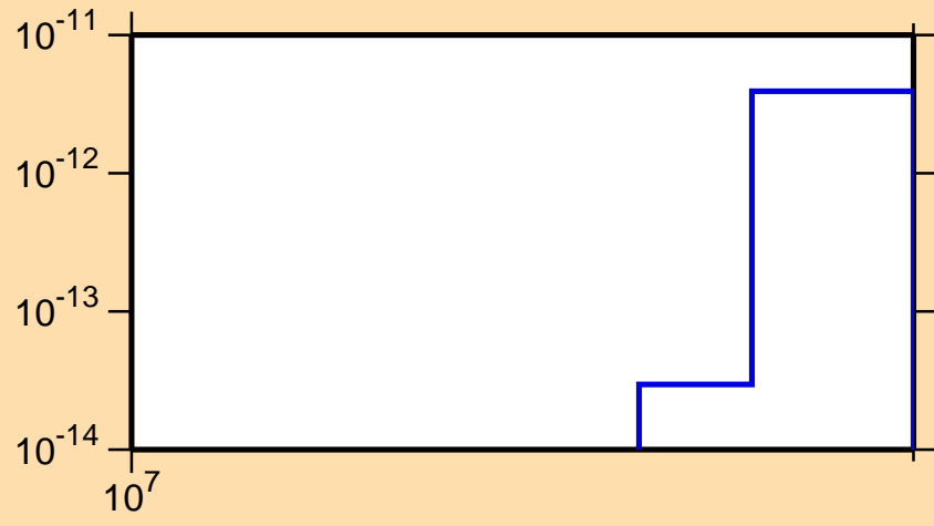
\sigma vs. E for ^{143}\text{Ce}(\text{mt117})
