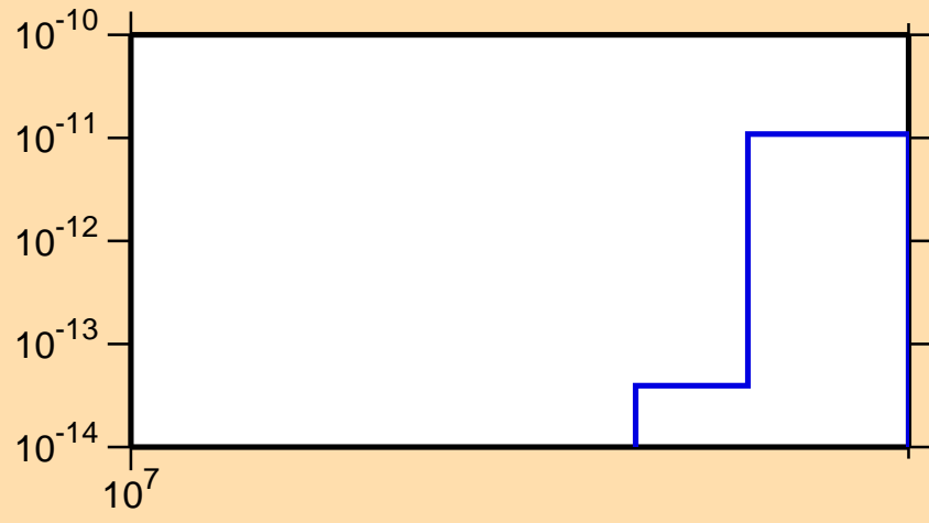
\sigma vs. E for ^{137}\text{La} (mt 45)
