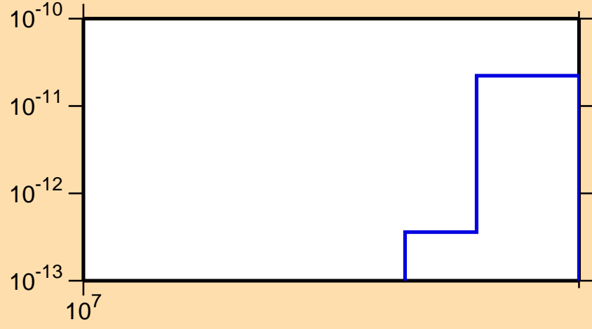
\sigma vs. E for ^{137}\text{La}(\text{mt117})
