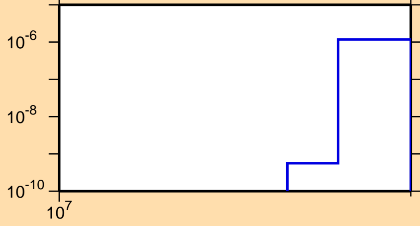
\sigma vs. E for ^{137}\text{La}(n,nt)
