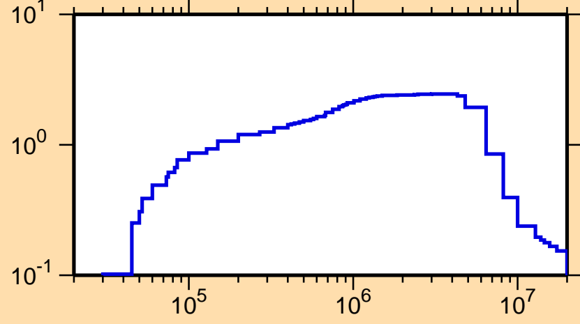
\sigma vs. E for ^{140}\text{La}(n,\text{inel.})
