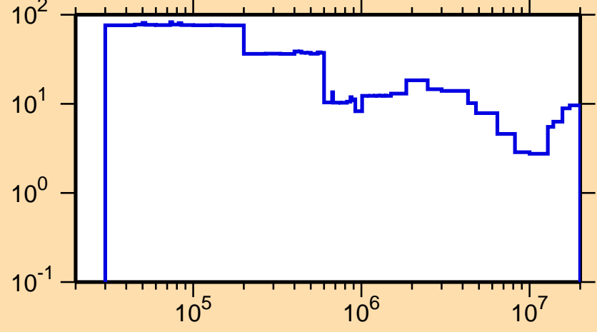
\Delta\sigma/\sigma vs. E for ^{140}\text{La}(n,\text{tot.})
