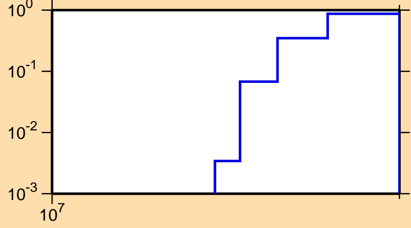
\sigma vs. E for ^{140}\text{La}(n,3n)
