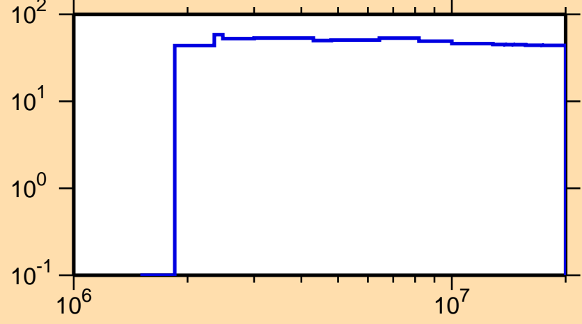
\Delta\sigma/\sigma vs. E for ^{140}\text{La}(n,p)
