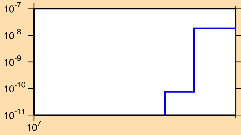
\sigma vs. E for ^{140}\text{La}(n,\text{He3})
