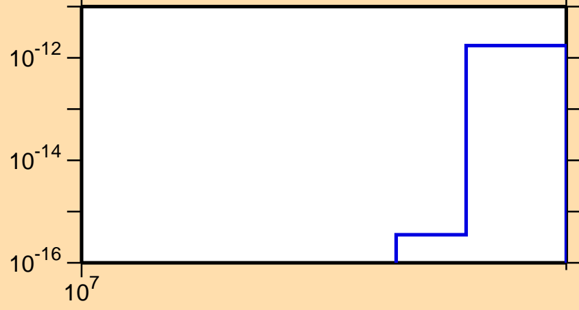
\sigma vs. E for ^{140}\text{La} (mt 34)
