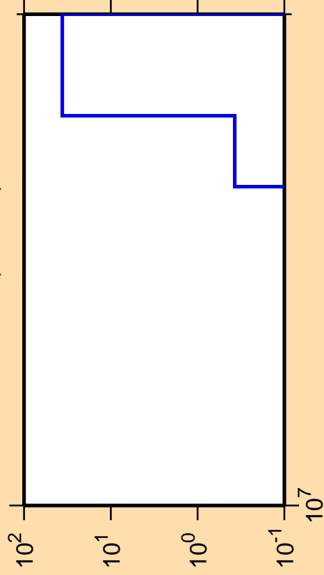
\Delta\sigma/\sigma vs. E for ^{140}\text{La}(\text{mt117})
