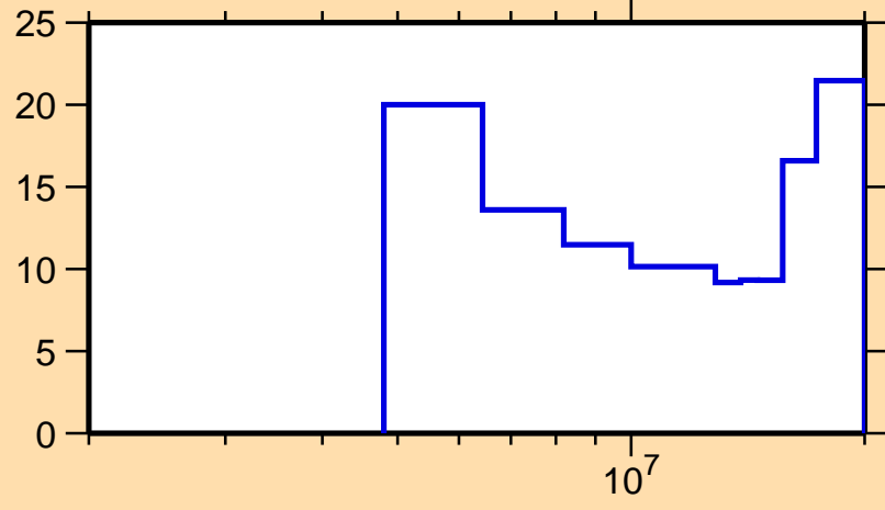
\Delta\sigma/\sigma vs. E for ^{140}\text{La}(n,2n)
