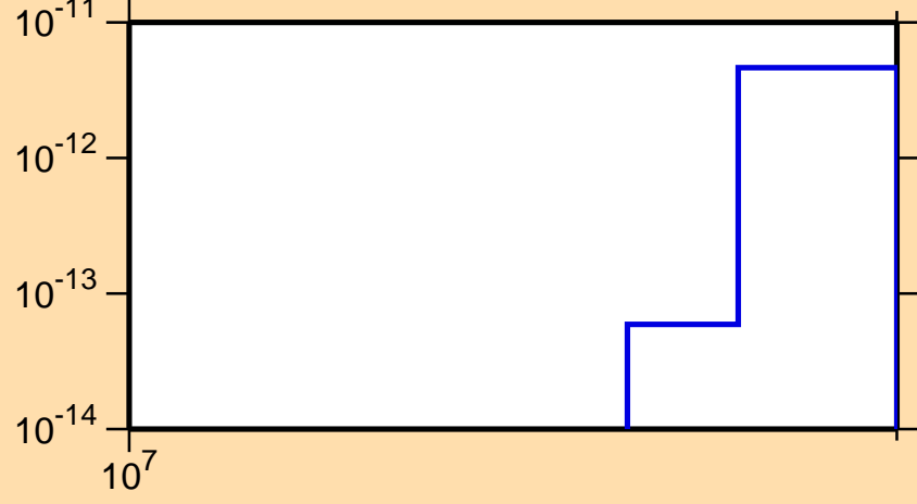
\sigma vs. E for ^{140}\text{La}(\text{mt117})
