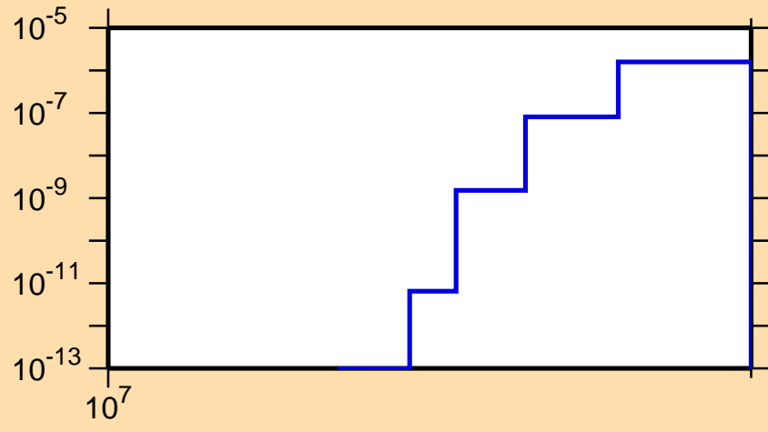
\sigma vs. E for ^{138}\text{La}(n,2n\alpha)
