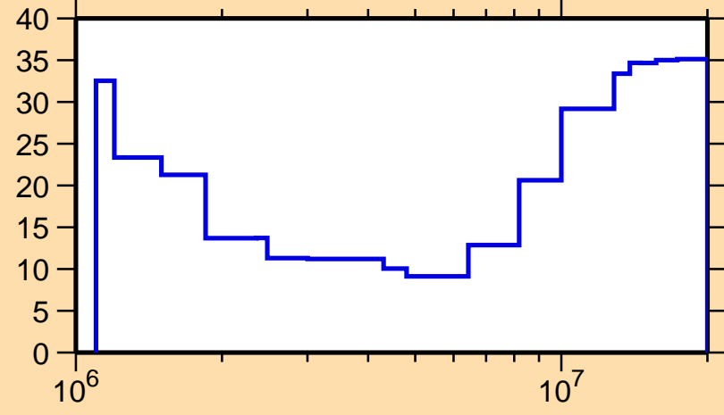
\Delta\sigma/\sigma vs. E for ^{138}\text{La}(n,n\text{cont.})
