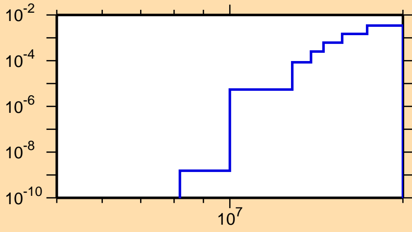
\sigma vs. E for ^{138}\text{La}(n,t)
