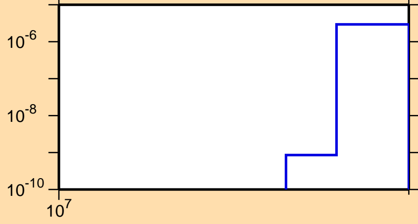
\sigma vs. E for ^{139}\text{Ba}(n,nt)
