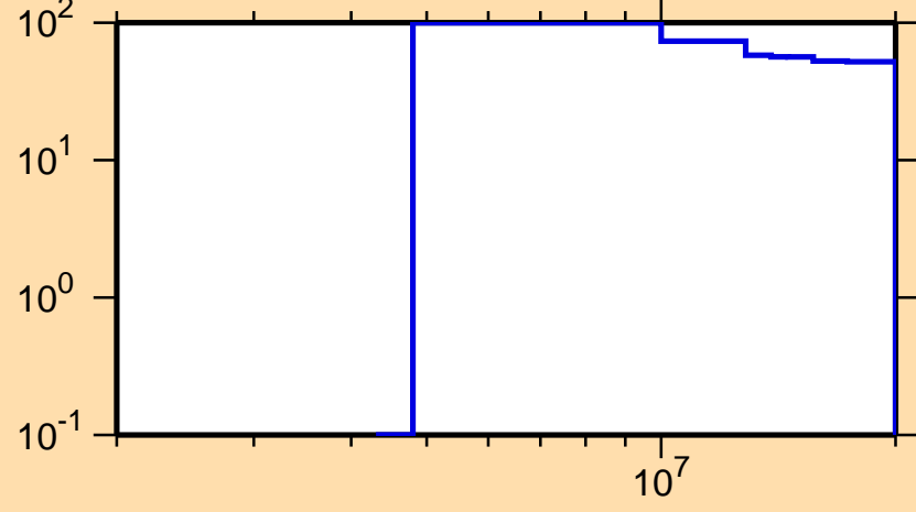
\Delta\sigma/\sigma vs. E for ^{139}\text{Ba}(n,p)
