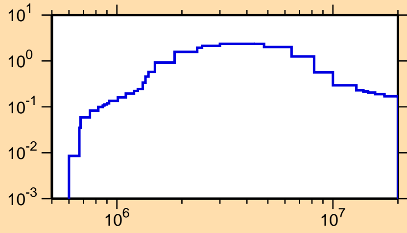
\sigma vs. E for ^{139}\text{Ba}(n,\text{inel.})
