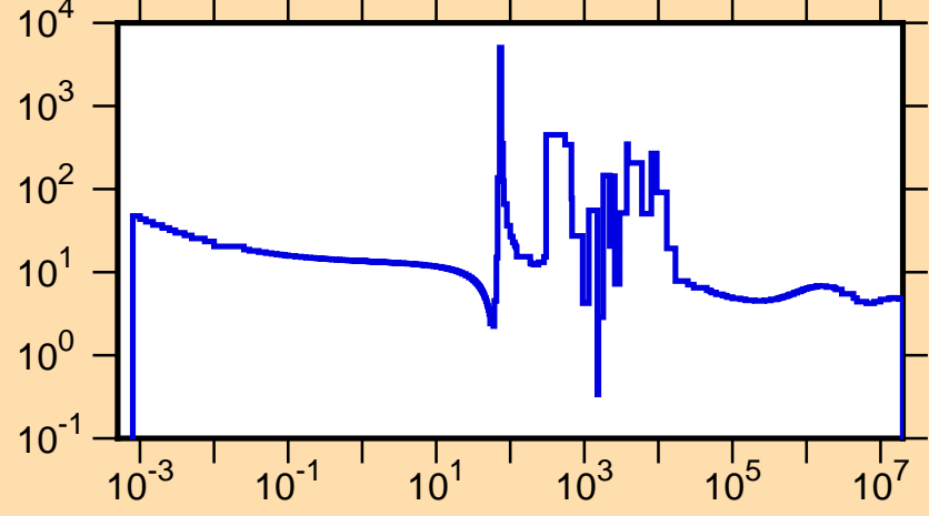
\sigma vs. E for ^{139}\text{Ba}(n,\text{tot.})
