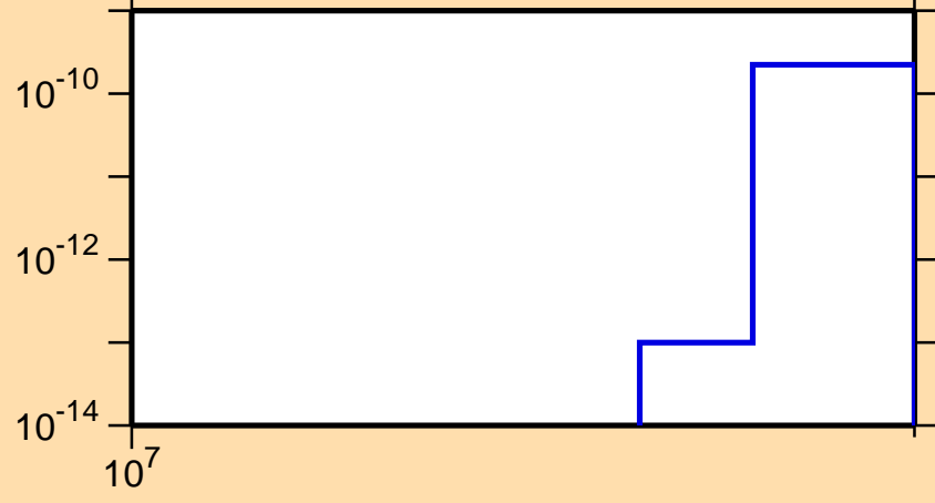
\sigma vs. E for ^{139}\text{Ba}(n,\text{He3})
