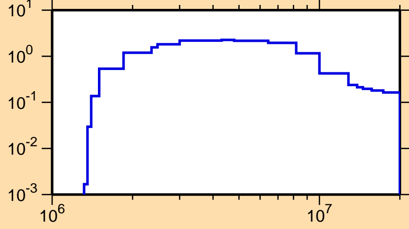
\sigma vs. E for ^{136}\text{Cs}(n,n\text{cont.})
