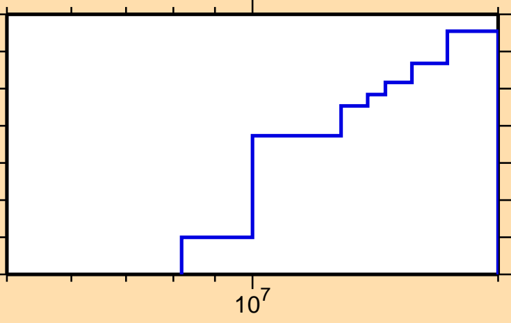
\sigma vs. E for ^{133}\text{Ba}(n,p\alpha)
