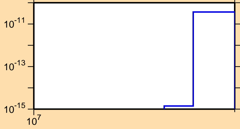
\sigma vs. E for ^{133}\text{Ba}(n,\text{pt})
