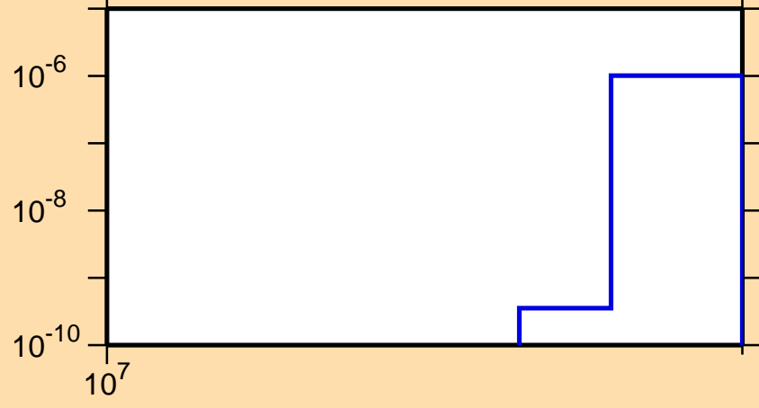
\sigma vs. E for ^{137}\text{Cs}(n,nt)
