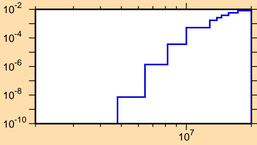
\sigma vs. E for ^{137}\text{Cs}(n,p)
