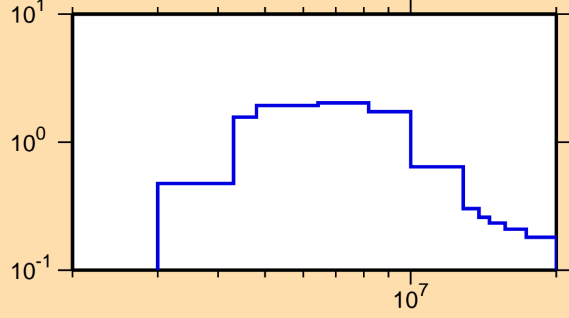
\sigma vs. E for ^{137}\text{Cs}(n,n\text{cont.})
