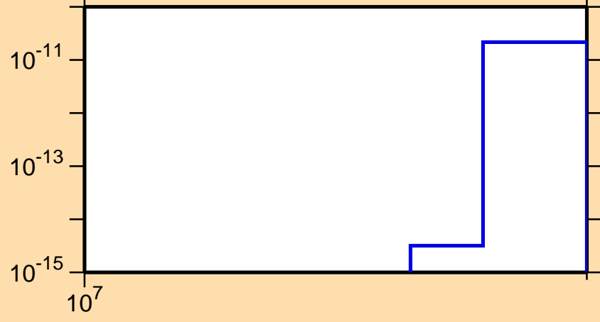
\sigma vs. E for ^{127}\text{Xe}(n,\text{pd})
