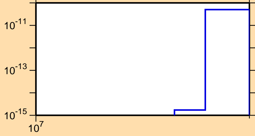
\sigma vs. E for ^{127}\text{Xe}(n,\text{pt})
