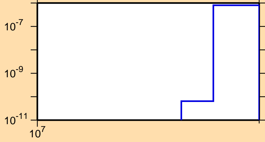
\sigma vs. E for ^{124}\text{Xe}(n,\text{nd})
