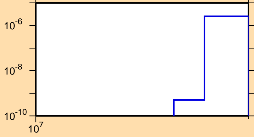
\sigma vs. E for ^{126}\text{I}(n,nt)
