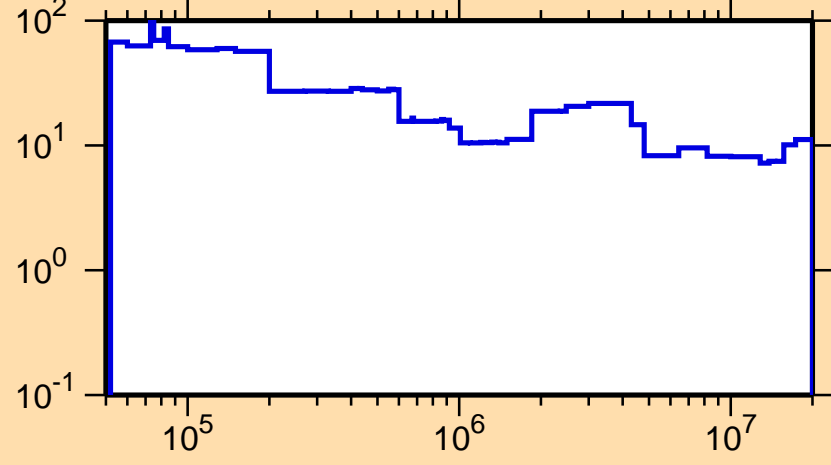
\Delta\sigma/\sigma vs. E for ^{126}\text{I}(n,\text{el.})
