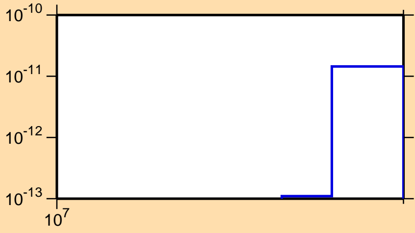
\sigma vs. E for ^{126}\text{I}(\text{mt117})
