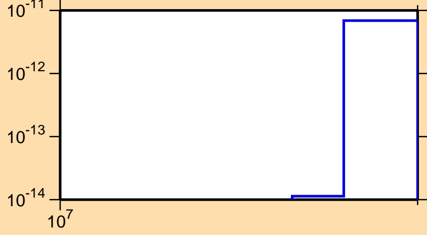
\sigma vs. E for ^{126}\text{I} (mt 45)
