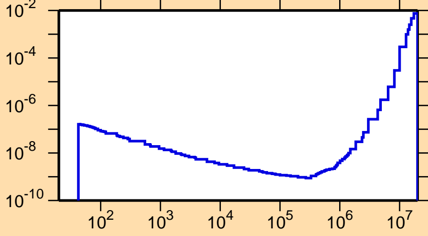
\sigma vs. E for ^{127}\text{Te}(n,\alpha)
