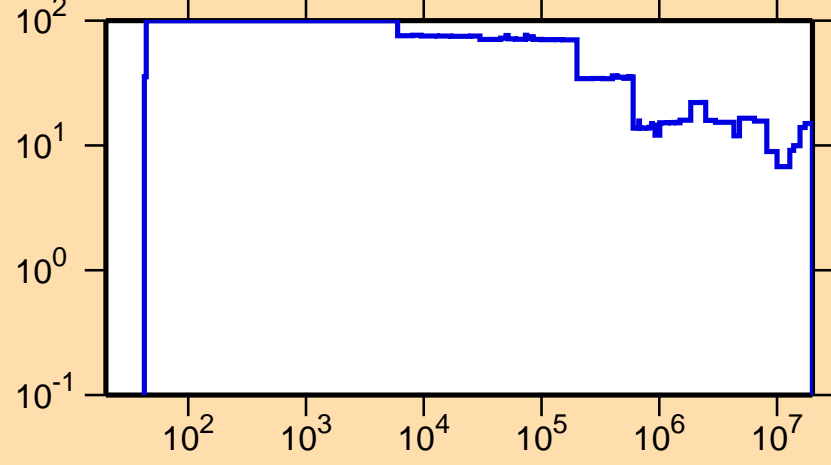
\Delta\sigma/\sigma vs. E for ^{127}\text{Te}(n,\text{el.})
