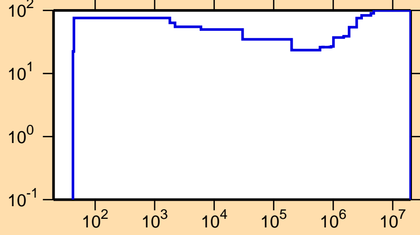
\Delta\sigma/\sigma vs. E for ^{127}\text{Te}(n,n_1)
