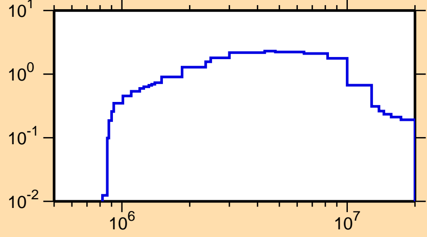
\sigma vs. E for ^{130}\text{Te}(n,\text{inel.})
