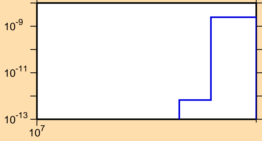
\sigma vs. E for ^{130}\text{Te}(n,2n\alpha)
