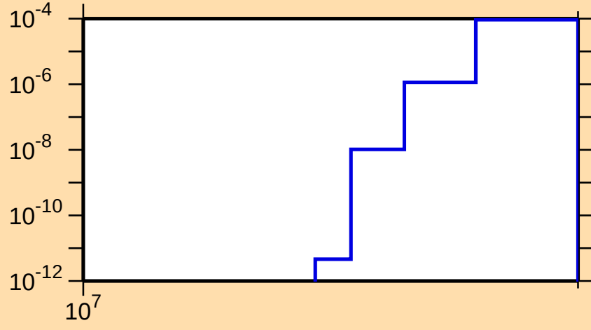
\sigma vs. E for ^{121}\text{Te}(n,\text{nd})
