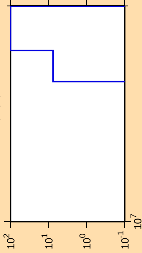
\Delta\sigma/\sigma vs. E for ^{121}\text{Te}(n,\text{pt})
