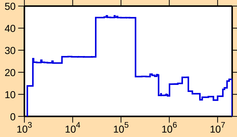
\Delta\sigma/\sigma vs. E for ^{121}\text{Te}(n,\text{el.})
