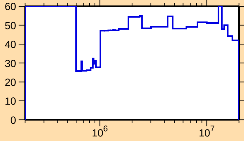
\Delta\sigma/\sigma vs. E for ^{121}\text{Te}(n,n_1)
