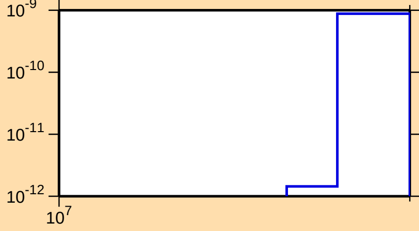
\sigma vs. E for ^{121}\text{Te}(n,\text{pd})
