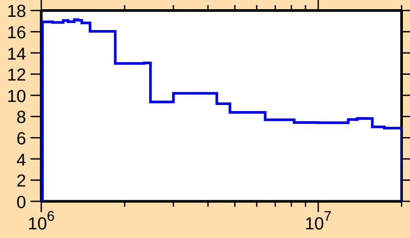
\Delta\sigma/\sigma vs. E for ^{121}\text{Te}(n,n\text{onel.})
