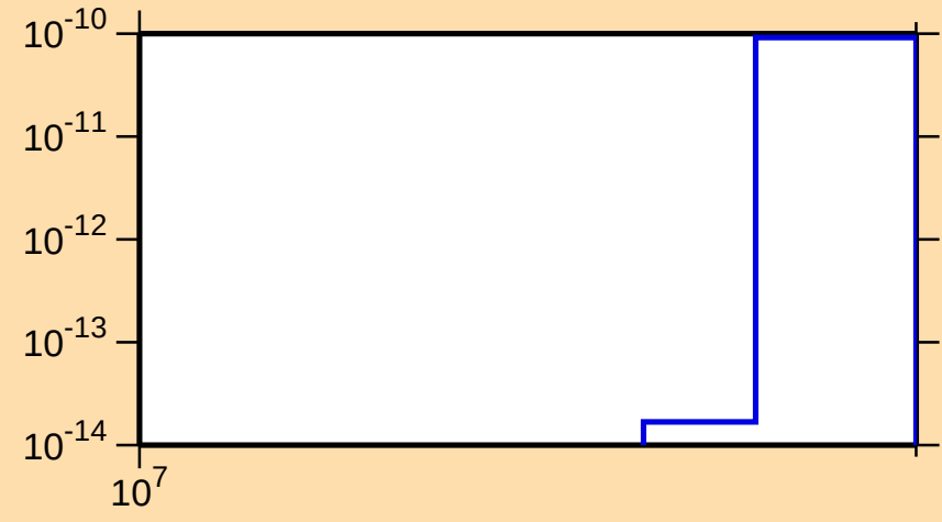
\sigma vs. E for ^{121}\text{Te}(\text{mt } 34)
