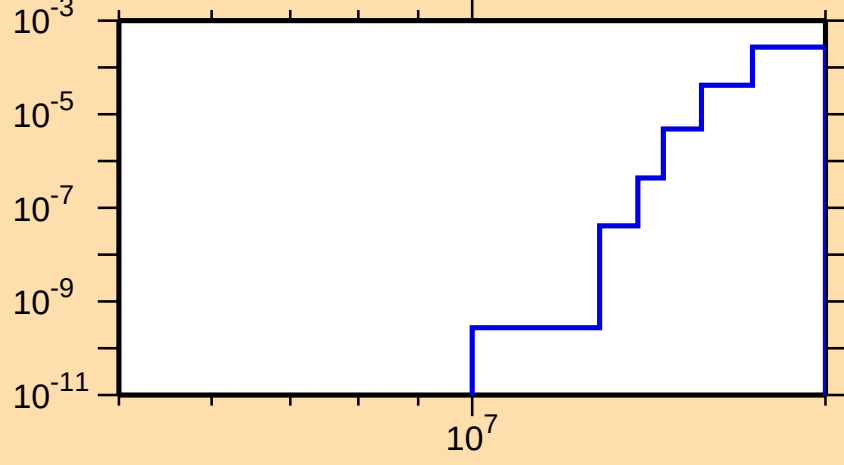
\sigma vs. E for ^{121}\text{Te}(n,2n\alpha)
