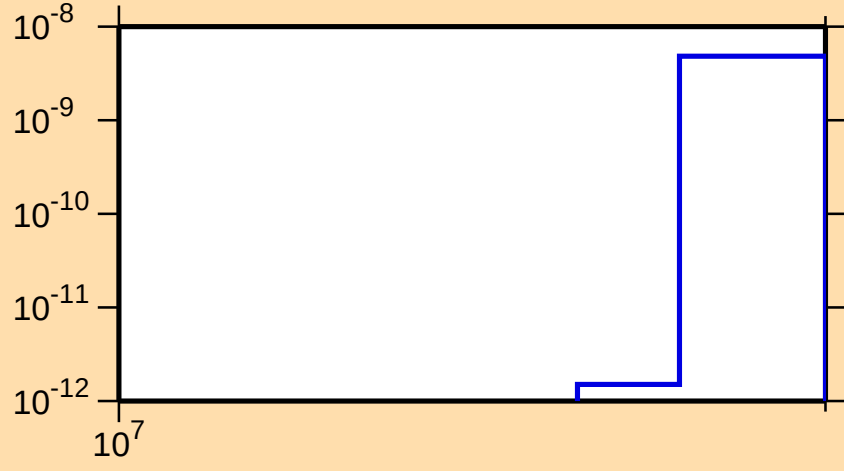
\sigma vs. E for ^{121}\text{Te}(n,\text{pt})
