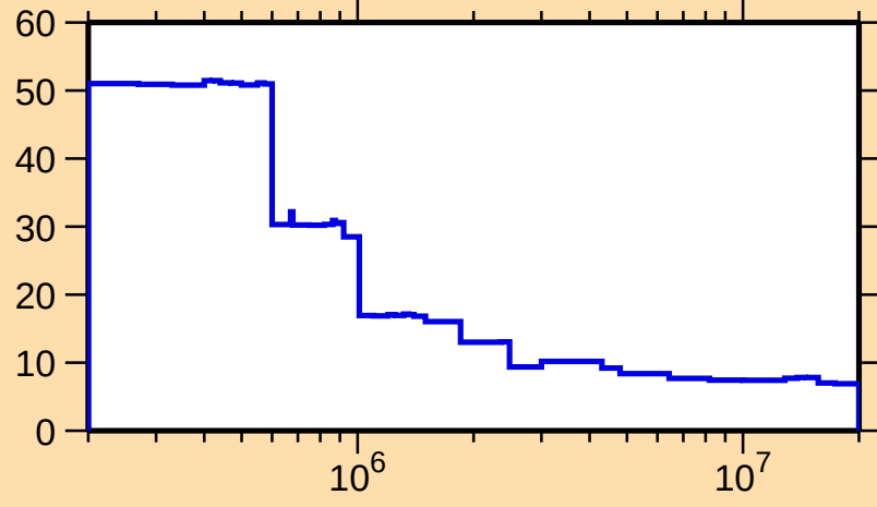
\Delta\sigma/\sigma vs. E for ^{121}\text{Te}(n,\text{nonel.})
