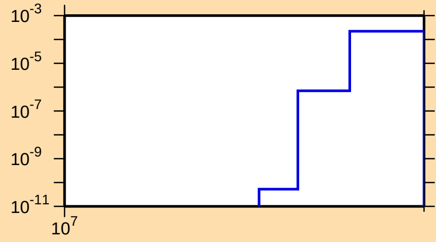
\sigma vs. E for ^{121}\text{Te}(n,2np)
