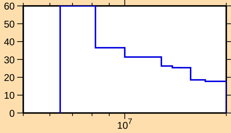
\Delta\sigma/\sigma vs. E for ^{121}\text{Te}(n,2n)
