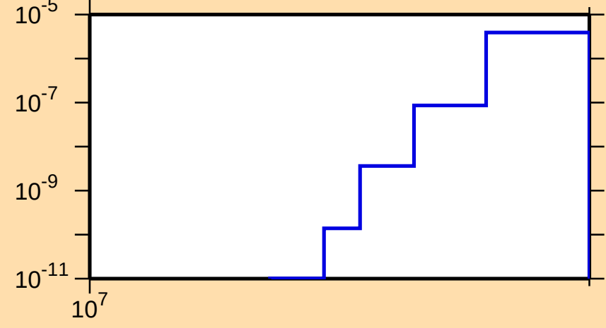
\sigma vs. E for ^{121}\text{Te}(n,\text{He3})
