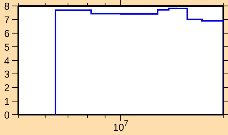
\Delta\sigma/\sigma vs. E for ^{121}\text{Te}(n,\text{nonel.})
