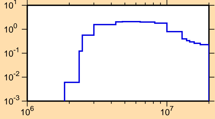
\sigma vs. E for ^{125}\text{Sb}(n,n\text{cont.})
