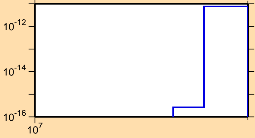
\sigma vs. E for ^{127}\text{Sb}(n,2n\alpha)
