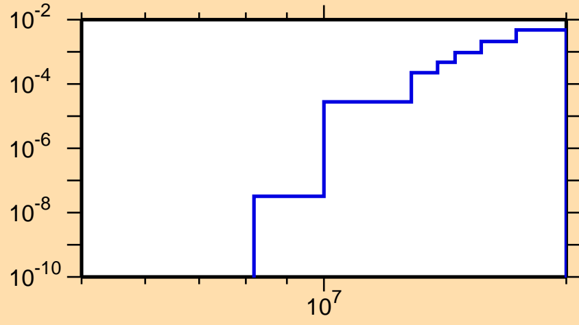
\sigma vs. E for ^{127}\text{Sb}(n,d)
