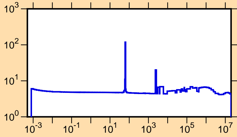
\sigma vs. E for ^{124}\text{Sn}(n,\text{tot.})
