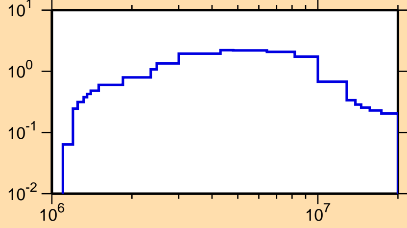
\sigma vs. E for ^{124}\text{Sn}(n,\text{inel.})
