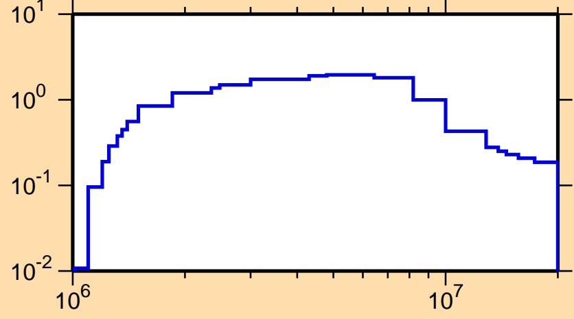
\sigma vs. E for ^{114}\text{In}(n,n\text{cont.})
