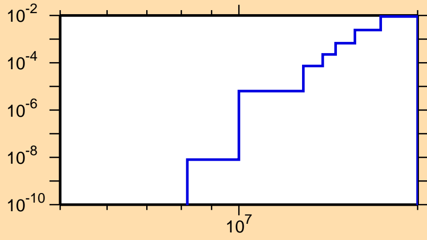
\sigma vs. E for ^{114}\text{In}(n,n\alpha)
