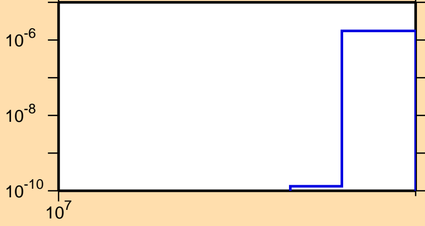
\sigma vs. E for ^{114}\text{In}(n,nt)
