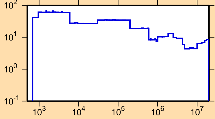
\Delta\sigma/\sigma vs. E for ^{114}\text{In}(n,\text{tot.})
