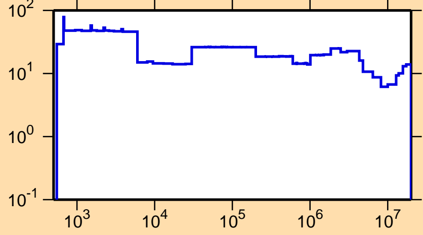
\Delta\sigma/\sigma vs. E for ^{109}\text{Cd}(n,\text{el.})
