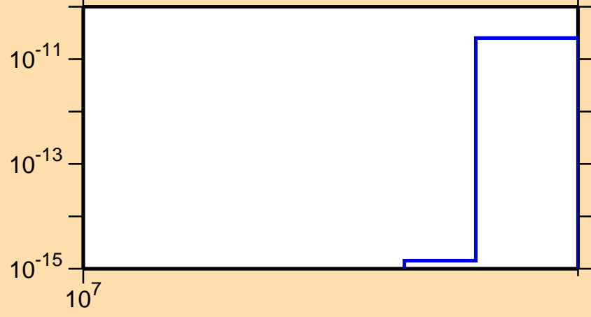
\sigma vs. E for ^{109}\text{Cd}(n,\text{pd})
