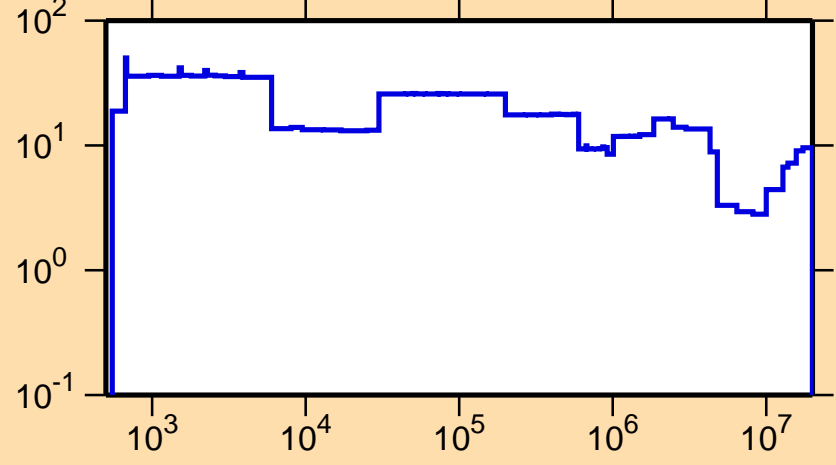
\Delta\sigma/\sigma vs. E for ^{109}\text{Cd}(n,\text{tot.})
