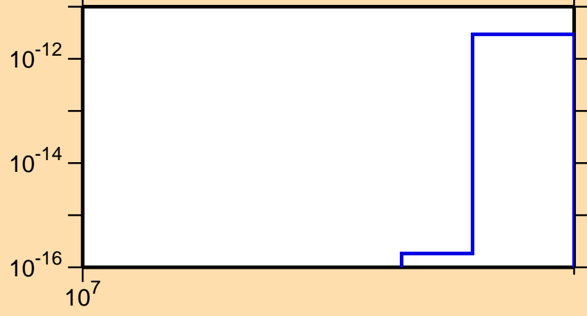
\sigma vs. E for ^{109}\text{Cd}(\text{mt } 34)
