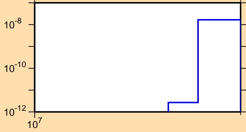
\sigma vs. E for ^{111}\text{Ag}(n,2n\alpha)
