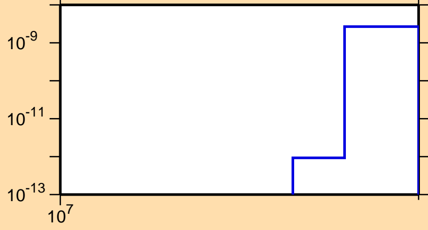
\sigma vs. E for ^{105}\text{Rh}(n,\text{He3})
