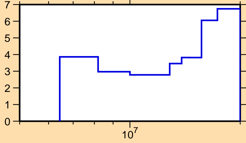
\Delta\sigma/\sigma vs. E for ^{110}\text{Ag}(n,\text{tot.})
