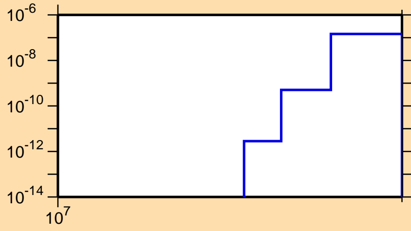
\sigma vs. E for ^{110}\text{Ag}(n,\text{He}3)
