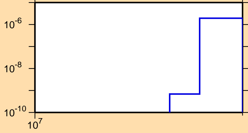
\sigma vs. E for ^{102}\text{Pd}(n,2n\alpha)
