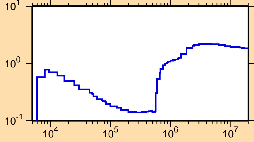
\sigma vs. E for ^{102}\text{Pd}(n,\text{nonel.})
