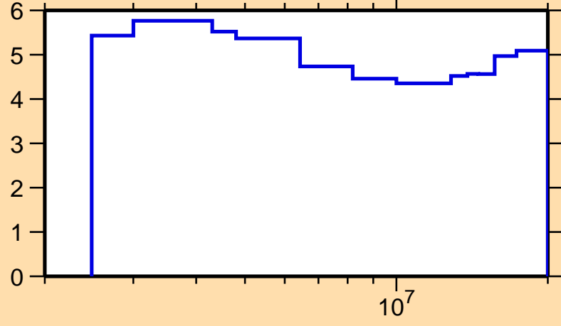
\Delta\sigma/\sigma vs. E for ^{102}\text{Pd}(n,n\text{inel.})
