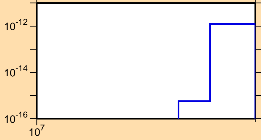
\sigma vs. E for ^{104}\text{Rh}(\text{mt117})
