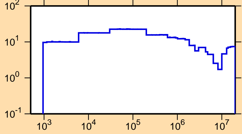
\Delta\sigma/\sigma vs. E for ^{104}\text{Rh}(n,\text{tot.})
