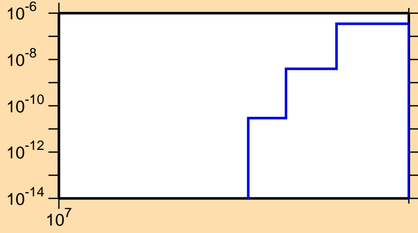
\sigma vs. E for ^{99}\text{Rh}(n,pd)
