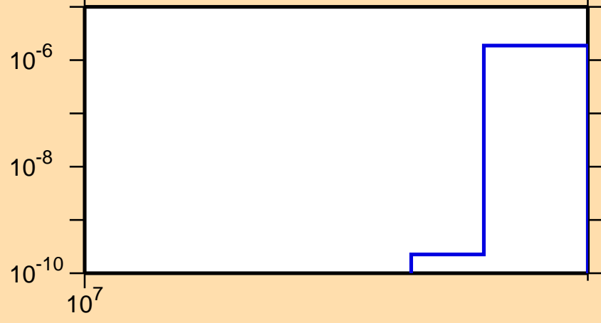
\sigma vs. E for ^{99}\text{Rh}(n,nt)
