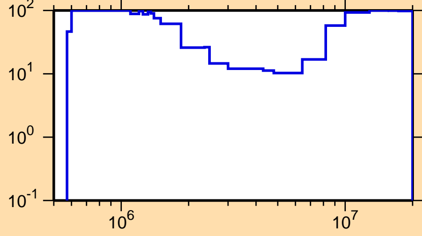
\Delta\sigma/\sigma vs. E for ^{96}\text{Tc}(n,n\text{cont.})
