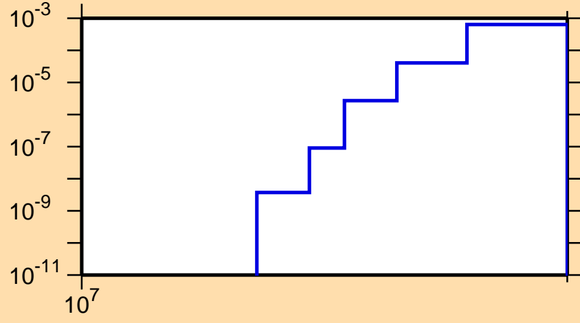
\sigma vs. E for ^{96}\text{Tc}(n,nd)
