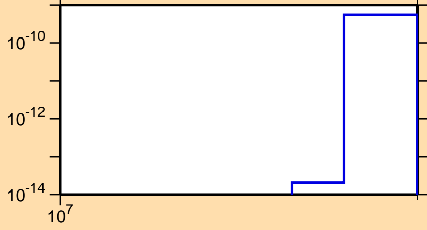
\sigma vs. E for ^{96}\text{Tc} (mt 34)
