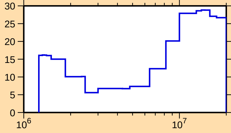
\Delta\sigma/\sigma vs. E for ^{99}\text{Mo}(\text{n},\text{inel.})
