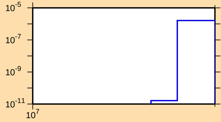
\sigma vs. E for ^{99}\text{Mo}(n,\text{nt})
