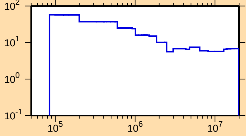
\Delta\sigma/\sigma vs. E for ^{99}\text{Mo}(n,\text{nonel.})
