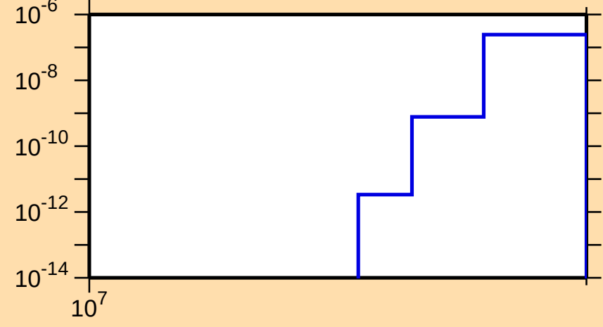
\sigma vs. E for ^{99}\text{Mo}(n,\text{He3})
