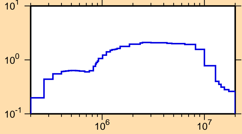
\sigma vs. E for ^{95}\text{Mo}(n,\text{inel.})
