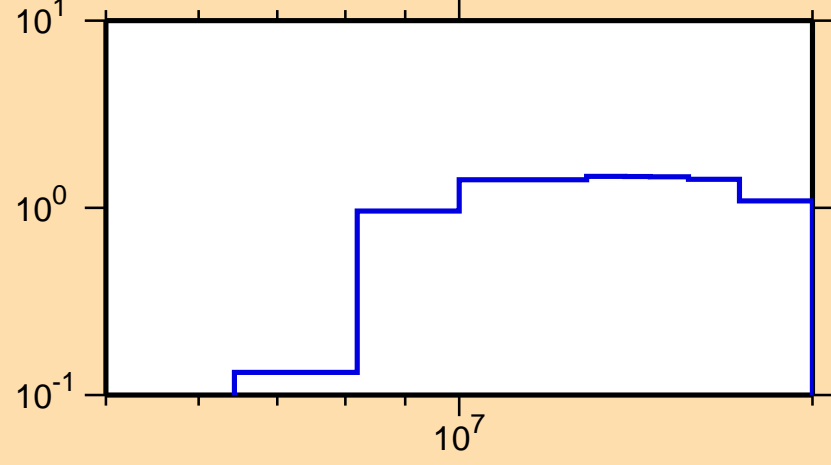
\sigma vs. E for ^{94}\text{Nb}(n,2n)
