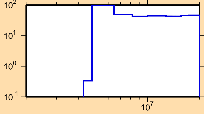
\Delta\sigma/\sigma vs. E for ^{95}\text{Zr}(n,p)
