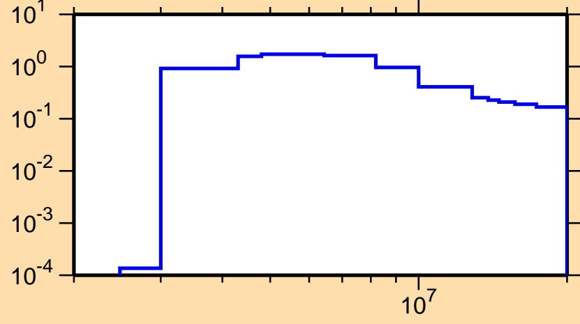
\sigma vs. E for ^{95}\text{Zr}(n,n\text{cont.})
