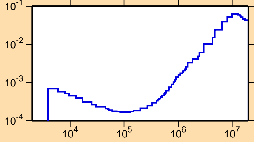
\sigma vs. E for ^{91}\text{Nb}(n,p)
