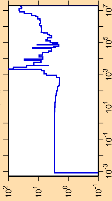
\Delta\sigma/\sigma vs. E for ^{89}\text{Y}(n,\gamma)
