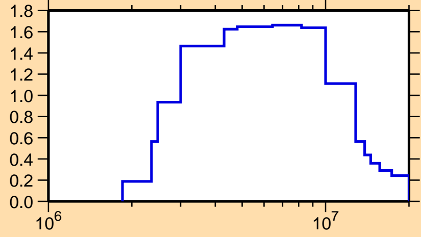
\sigma vs. E for ^{88}\text{Y}(n,n\text{cont.})
