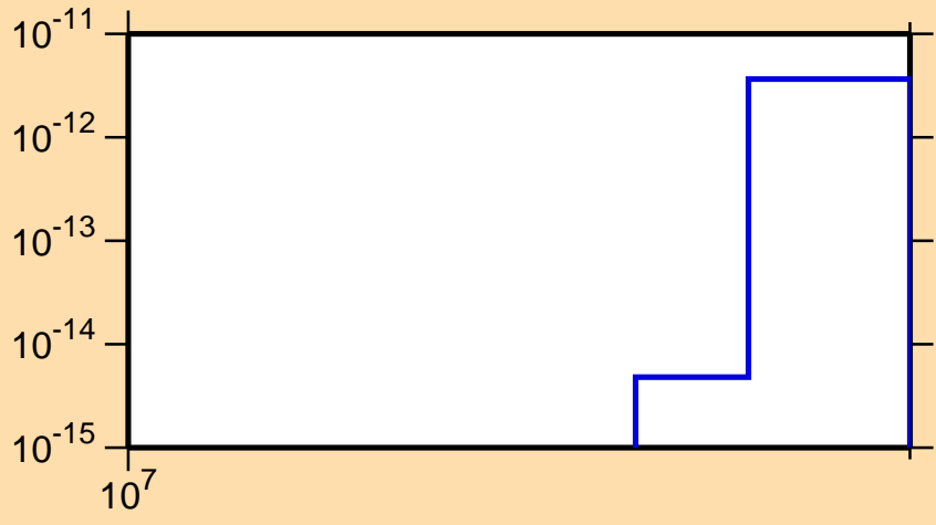
\sigma vs. E for ^{88}\text{Y}(n,2n\alpha)
