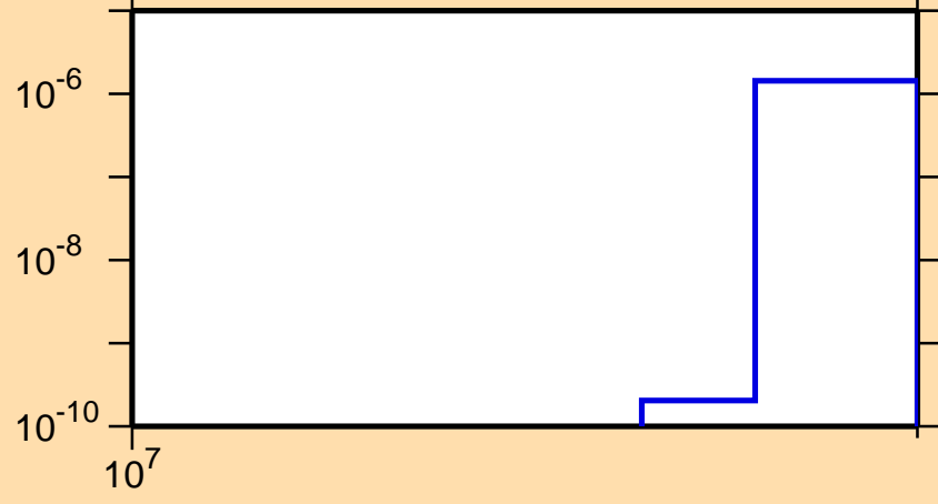
\sigma vs. E for ^{83}\text{Sr}(n,2n\alpha)
