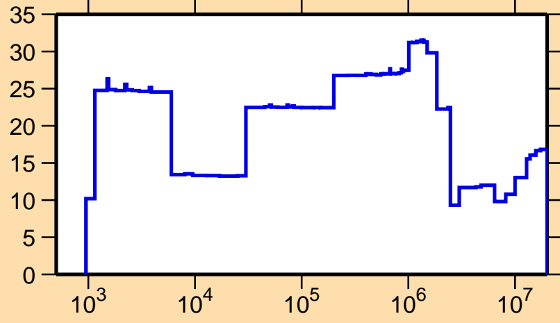
\Delta\sigma/\sigma vs. E for ^{83}\text{Sr}(n,el.)
