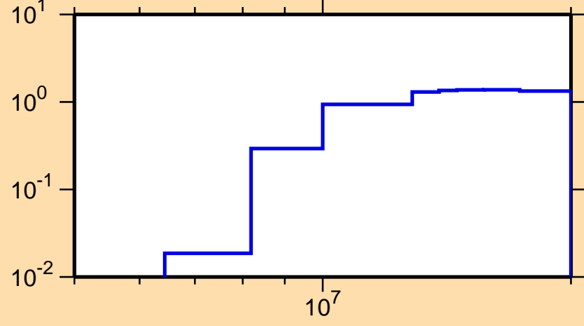
\sigma vs. E for ^{85}\text{Kr}(n,2n)
