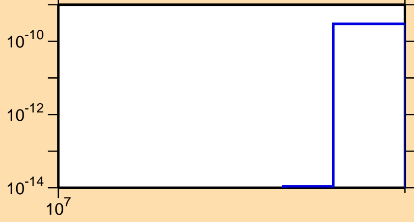
\sigma vs. E for ^{85}\text{Kr}(n,2n\alpha)
