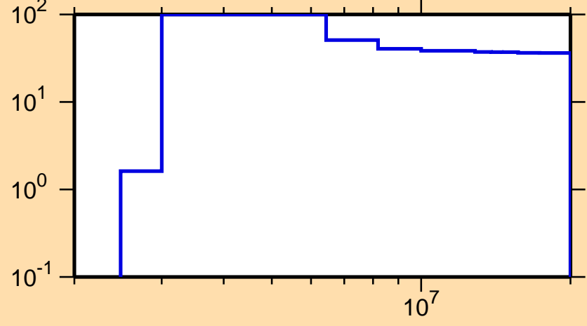
\Delta\sigma/\sigma vs. E for ^{85}\text{Kr}(n,p)
