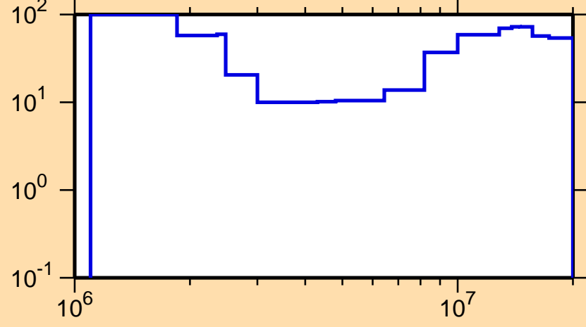
\Delta\sigma/\sigma vs. E for ^{77}\text{Br}(n,ncont.)
